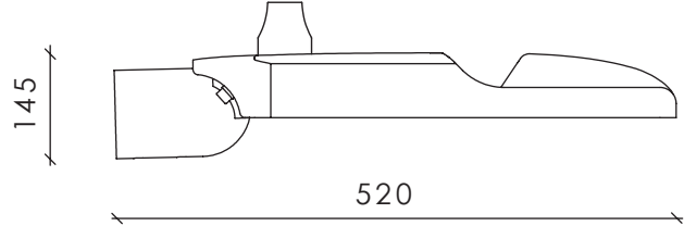
Dimensions with RF antenta
