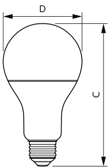
Bulb A67 14-100W 1521lm 2700-2200K E27 D
